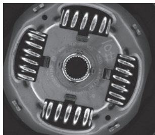
Small spring presence detection in large spring
