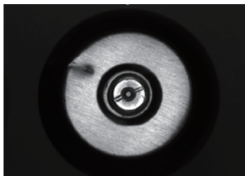
Defect detection of oral liquid bottle cap: Defects on curved surfaces can be illuminated under spot light.
