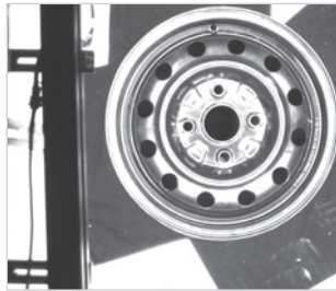
Wheel hub surface stain detection and dimension detection
