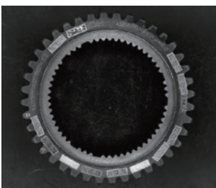
Gear tooth space width barcode detection
