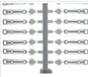
Glucometer needle presence detection
